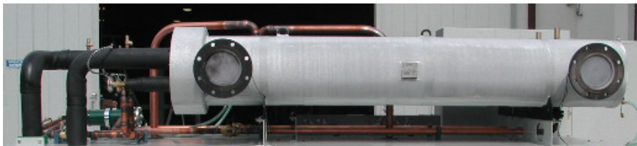
Evaporatore fascio tubiero - Shell and tube evaporator
