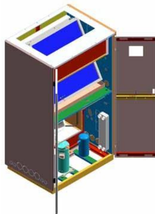
TECHNICAL COMPARTMENT Positioned in the lower section for easiest maintenance
